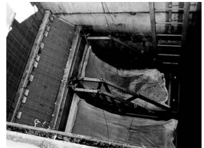
In-system netting can provide floatables control at strategic locations in the sewer system.
